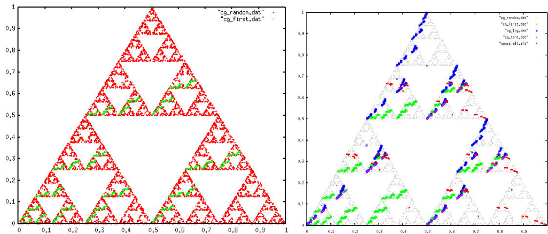
FIG. 11: (Left panel) IFS chaos game-like attractor for the type I null model with p = 3 symbols. In this case the attractor is the Sierpinski triangle. (Right panel) IFS chaos game-like attractor for the prime gap sequence and a symbolic sequence extracted from other chaotic maps. The IFS associated to the prime gap sequence is a subset of the attractor. The similarity with the tent map is again notable, where in this case the attractor of the tent map is a subset of the attractor of the prime gap sequence. As a comparison, we have included a different chaotic map (the Gauss map) which shows no similarities with the gaps.
