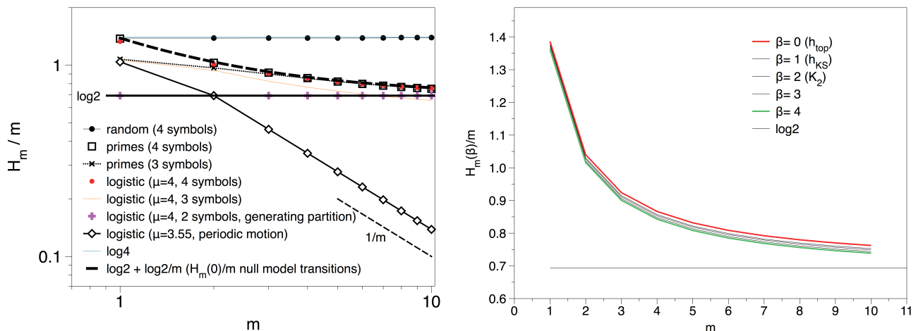
FIG. 6: (Left) Block entropies H_m(1)/m for different symbolic sequences. (Right) Renyi block entropies H_m(\beta)/m for different values of m and \beta . All curves seem to converge to \log 2 .
