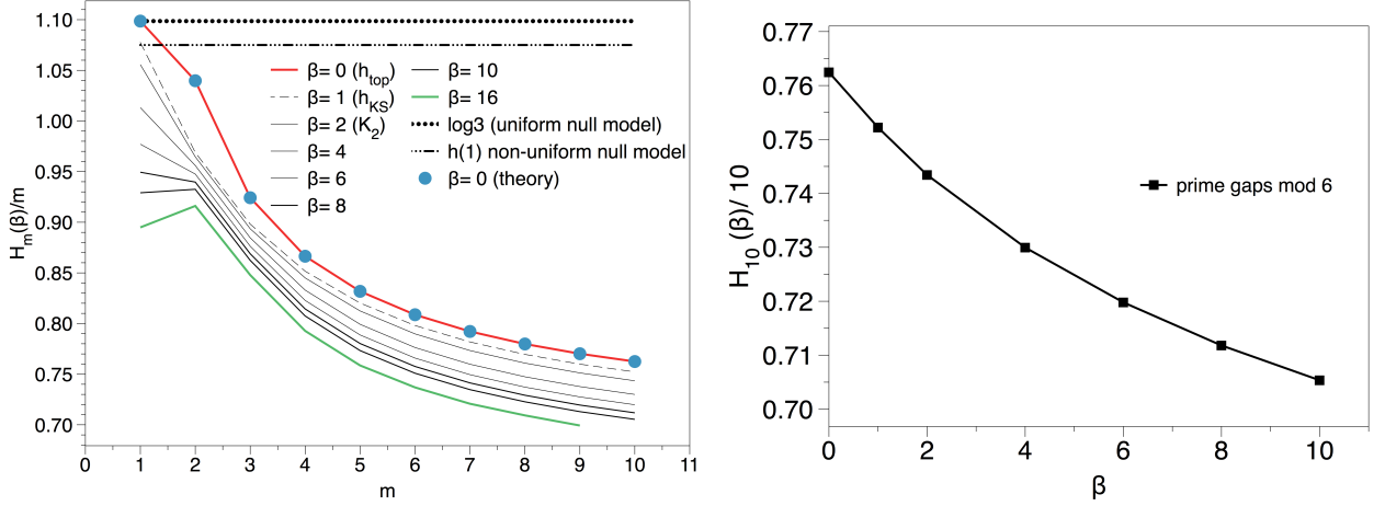
FIG. 10: (Left panel) H_m(\beta)/m associated to the primes gaps modulo 6. (Right panel) Spectrum of Renyi entropies associated to the primes gaps modulo 6.
