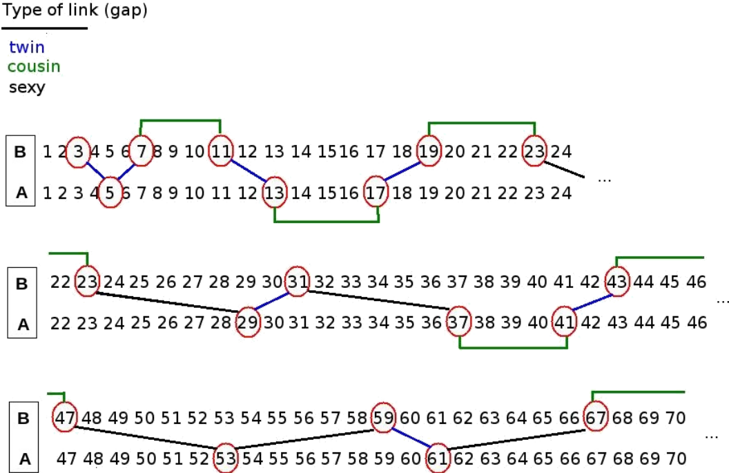
FIG. 4: Transitions between consecutive primes, labelled in terms of twins, cousins and sexies.
