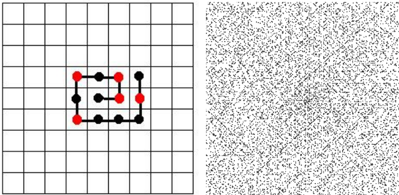
FIG. 1: (left)The Ulam spiral for the sequence 1, 2 ... 12, with primes in red. (right) A full 200 x 200 Ulam spiral showing the primes as individual black dots. Notice the emergent diagonal pattern where the primes tend to accumulate.
