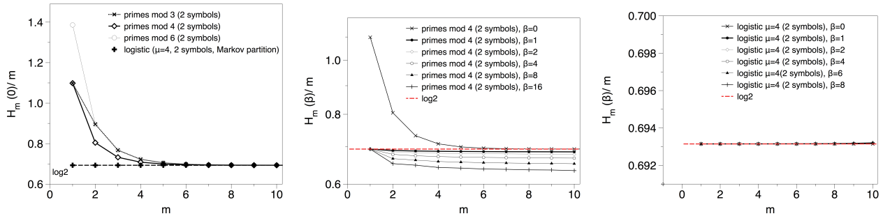
FIG. 8: (Left) Block entropies H_m(0)/m for symbolic sequences primes mod k , with different values of k . We find that the topological entropy is always \log 2 , suggesting that there are no forbidden patterns in primes modulo k . (Middle) Empirical Renyi block entropies H_m(\beta)/m for different values of m and \beta , extracted from the primes modulo 4. The spectrum does not collapse into a single value. (Right) Empirical Renyi block entropies H_m(\beta)/m for different values of m and \beta , extracted from the fully chaotic logistic map x_{t+1} = 4x_t(1 - x_t) after symbolization with p = 2 symbols. Results have been computed over a symbolic sequence of N = 10^6 points, the same size as the one for the primes in the middle and left panels. The spectrum in this case collapses h(\beta) = \log 2, \forall \beta as expected according to the topological conjugacy of the fully chaotic logistic map with the binary shift.
