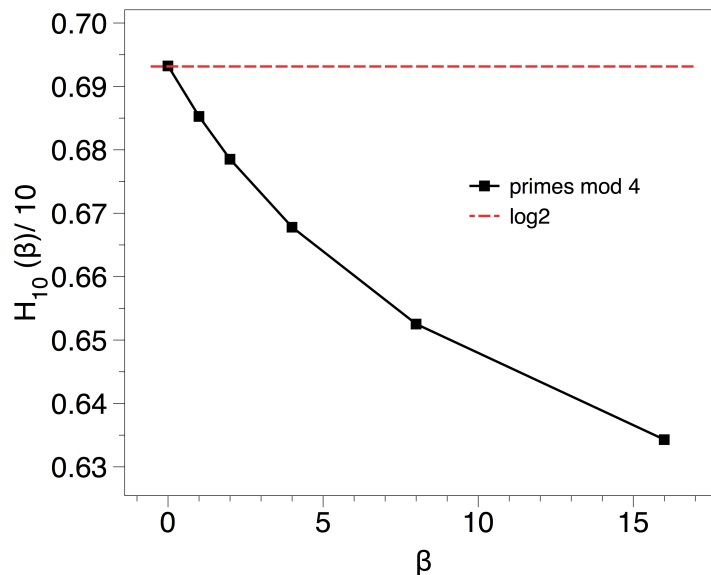
FIG. 9: Spectrum of Renyi entropies associated to the primes modulo 4.
