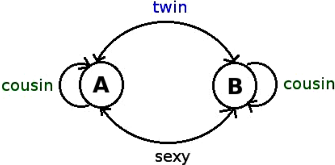
FIG. 3: A network representation of the prime numbers sequence and state transitions. Prime sequence can be seen as the result of a Markov Chain defined over a two-state network with certain transition rates. In figure 4 we depict an illustration of such a Markov Chain process.
