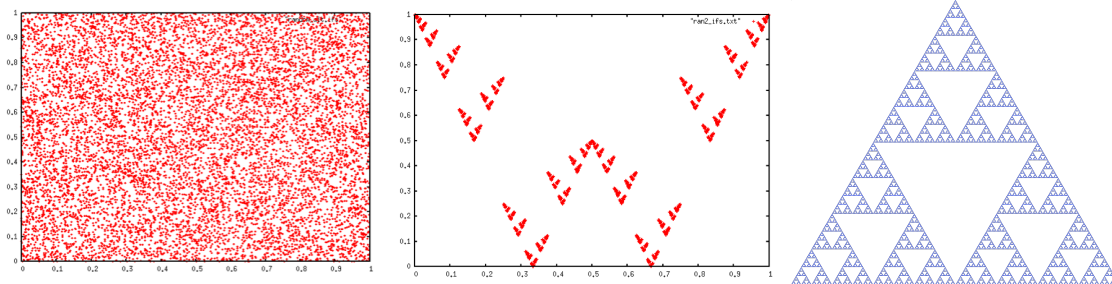
FIG. 5: IFS attractor for (left panel) a type I null model with p = 4 symbols, (middle panel) a type II null model with p = 4 symbols, (right panel) a type I null model with p = 3 symbols.
