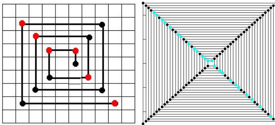
FIG. 2: (Left panel) The diagonal spiral for the sequence 1, 2 ... 13, with primes in red. (Right panel) The diagonal spiral for N = \{2 \dots 100\} , with primes in blue. The upper-left spiral arm agglutinates primes of the form 4n + 3 , called Gaussian primes. The bottom-right agglutinates the rest of the primes with form 4n + 1 , called Pythagorean primes.
