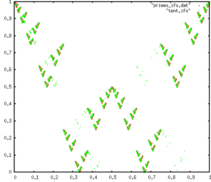
FIG. 7: IFS chaos game-like attractor for the prime transition sequence. The attractor has a fractal shape instead of being space-filling, however a type II null model can account for such shape, as shown in figure 5.
