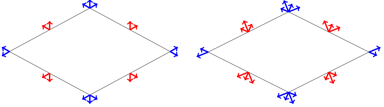
FIGURE 5. The sets R(F) for the faces F of the cube in type A_2 (left) and B_2 (right). Note that positive roots point downwards.
