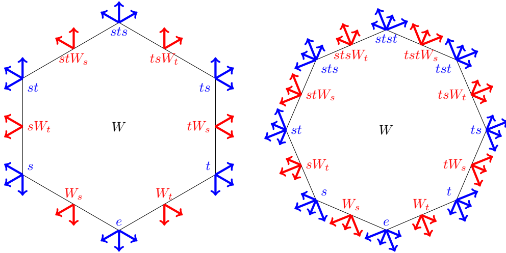
FIGURE 3. The sets R(xW_I) of the standard parabolic cosets xW_I in type A_2 (left) and B_2 (right). Note that positive roots point downwards.
