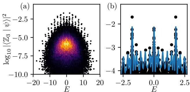
Figure 5. (a) The overlap between eigenstates of the PXP model and |\mathbb{Z}_3\rangle state as a function of energy E reveals another special band of eigenstates. (b) Same plot but zoomed in around energy E = 0 . Black dots mark individual eigenvalues, while the blue curve is a Gaussian convolution of the overlap probability |\langle \mathbb{Z}_3 | \psi(E) \rangle|^2 viewed as a function of energy. This reveals a number of peaks subdividing the interval between the highest overlap states. Both plots are for L = 30 in the zero-momentum and inversion symmetric sector together with the \pm 2\pi/3 momentum sectors.
