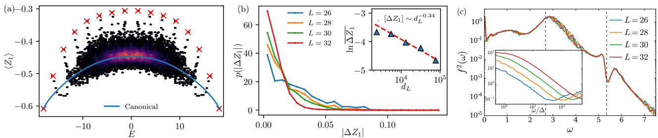
Figure 2. (a) Strong violation of the ETH revealed by the eigenstate expectation values \langle O^Z \rangle \equiv \langle Z_1 \rangle , plotted as function of energy (color scale indicates the density of data points). While the majority of points are concentrated in the vicinity of the canonical ensemble prediction, the band of special eigenstates (indicated by crosses) is also clearly visible. For these eigenstates, \langle O^Z \rangle strongly deviates from the canonical prediction at the corresponding energy. The system contains L = 30 atoms in the zero momentum, inversion-symmetric sector. (b) Probability distribution for the difference in expectation value of the local observable O^Z between eigenstates adjacent in energy. Inset: Mean \overline{\Delta O^Z} decays with a power \approx 1/3 of the Hilbert space dimension d_L^{\text{PBC}} as the system size is increased (shown up to L = 32 ). Averaging is performed over eigenstates in an interval between adjacent special states in the middle of the spectrum. The line shown is a linear regression to the three largest system sizes. (c) Off-diagonal matrix elements are a smooth function of the energy difference. Moreover, f^2(\omega) does not depend on the system size, consistent with the ETH. At the same time, a number of features are visible in f^2(\omega) at the frequency coinciding with the energy separation of special eigenstates in panel (a). The inset shows that f^2(\omega) , plotted as a function of energy in units of many-body level spacing \Delta , does not have a well-developed plateau until \omega \leq \Delta .
