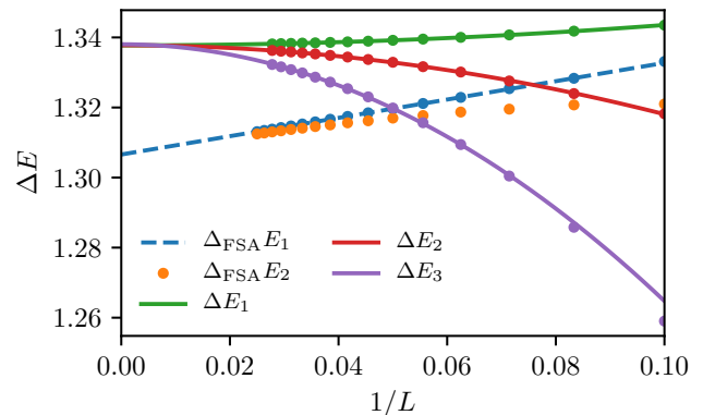
Figure 4. Finite size scaling of the energy gaps between special states closest to the middle of the spectrum shows the convergence of all gaps to the same value in the thermodynamic limit. Note that adjacent special states belong to different momentum sectors. The gaps accurately follow quadratic dependence on 1/L in the range of available system sizes L = 10, \dots, 36 . The prediction of the forward scattering approximation, discussed in Sec. IV for systems with up to L = 48 sites, is shown by blue/orange points, corresponding to the two states closest to the middle of the spectrum. Within this approximation, the energies appear to follow linear dependence in 1/L (dashed line).
