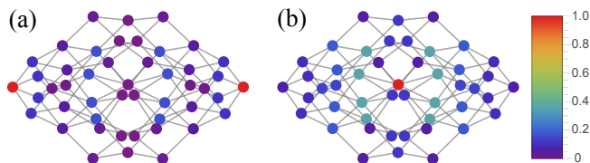
Figure 7. Two eigenstates of the PXP model represented on the Hilbert space graph for L = 10 sites and PBC. The color of the vertices reflects the weight of the corresponding product state in the eigenvector, where the largest weight is normalized to one. Similar to Fig. 1, the Néel states are the left/right most vertices of the graph, while the fully polarized state is located in the center of the graph. (a) Wave function of the special eigenstate closest to zero energy is concentrated in the vicinity of the Néel states. In contrast, the wave function of the ground state (b) is concentrated in the center of the graph.
