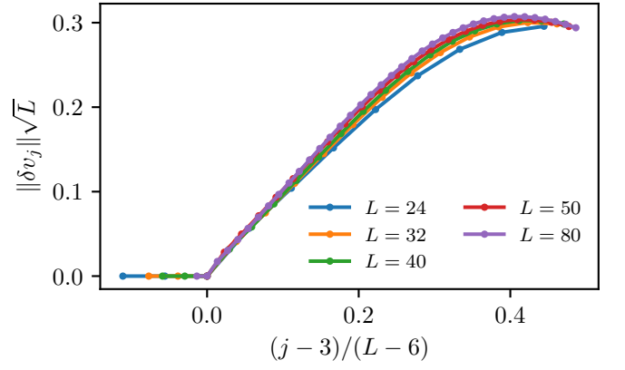
Figure 11. Normalized errors \|\delta v_j\| rescaled by a factor of \sqrt{L} for PBC in the parity symmetric sector. With this rescaling, the errors for different L are well collapsed, suggesting \|\delta v_j\|^2 = O(j^2/L^3) .
