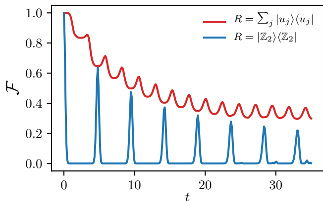
Figure 12. Red curve shows the time dependence of the probability to be found within the forward-scattering subspace, measured by Eq. (B3). Blue curve shows the fidelity for the Néel initial state. Data is for system size L = 32 .
