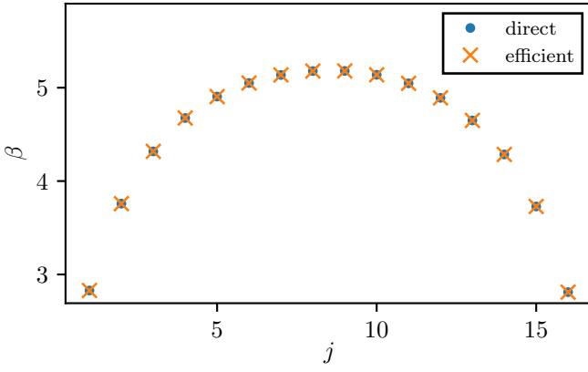
Figure 13. A demonstration of exact agreement between direct computation of \beta coefficients from Eq. (C1) and computation from the efficient recurrence, Eq. (C11). Data is for N = 16 site chain with open boundary conditions.
