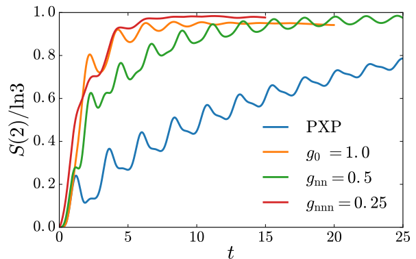
Figure 10. The dynamics of two-site entanglement in the quantum quench from |\mathbb{Z}_2\rangle initial state is strongly influenced by perturbations to the PXP model. We note that nearest-neighbor hopping is the least effective in damping the oscillations. In contrast, for the perturbation g_{\text{nnn}} = 0.25 , when the bulk of eigenstates becomes fully thermal, the oscillations in entanglement and local observables are strongly damped. The entanglement is normalized by the maximal possible value for two sites, which is equal to \ln 3 due to the presence of a constraint. The data is obtained with iTEBD, the maximal evolution time is limited by the bond dimension \chi = 1200 .
