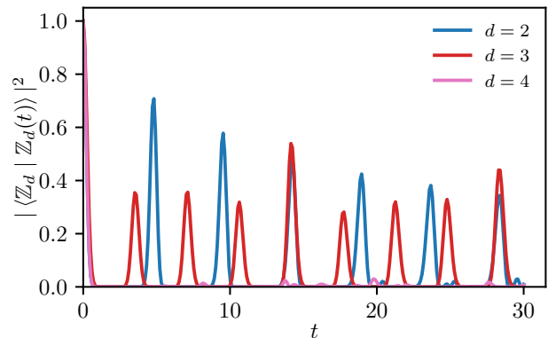
Figure 6. Quantum fidelity shows periodic in time revivals for |\mathbb{Z}_2\rangle and |\mathbb{Z}_3\rangle initial product states. In contrast, |\mathbb{Z}_4\rangle initial state shows a complete absence of revivals. Data is for system with L = 24 sites with periodic boundary conditions.
