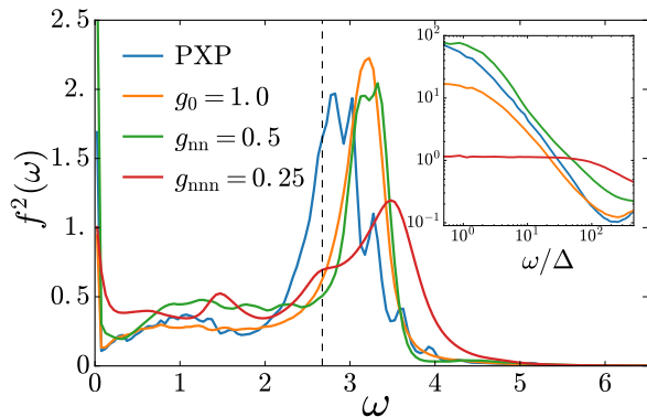
Figure 9. Peak in the energy dependence of matrix elements of the unperturbed PXP model at \omega \approx 2.66 softens and shifts upon the addition of perturbations. Moreover, the inset shows that the plateau in f^2(\omega) only slightly increases its size when the added perturbation is chemical potential or correlated hopping. In contrast, upon adding \delta H_{\text{nnn}} , the plateau increases to values of \omega/\Delta \leq 200 , fully consistent with the restoration of conventional thermalization.
