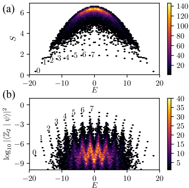
Figure 3. (a) Bipartite entanglement entropy of eigenstates, S , as a function of energy E . Region A is chosen as one half of the chain. The bulk of the states have large volume-law entropy ( S \gtrsim 5 ), however some outliers with anomalously low entropy ( S \lesssim 2 ) are also visible. These states are labelled by 0, \dots, 7 , and they span the entire energy range between the ground state (state 0) and the middle of the band (state 7). (b) Density plot showing the joint distribution of energy and overlap with |\mathbb{Z}_2\rangle product state among the energy eigenstates. The states with largest overlap are identified with the low entropy states from the top panel. Data shown is for L = 30 sites in the zero-momentum and inversion symmetric sector.
