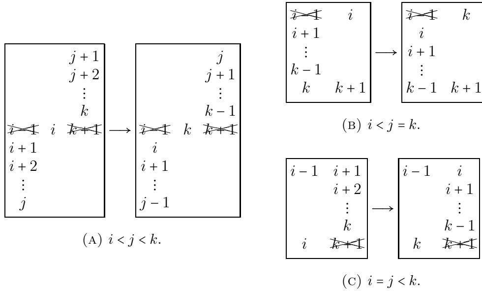
FIGURE 6. Summary diagrams for negative rotations.
