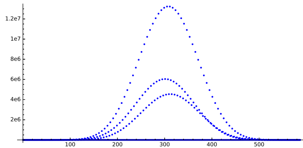
FIGURE 10. A plot of the coefficients for the deformed q -multinomial \left[ \begin{smallmatrix} n \\ \alpha \end{smallmatrix} \right]_{q;d} with \alpha = (2, 1, 3, 1, 4, 5) and d = 3 .
