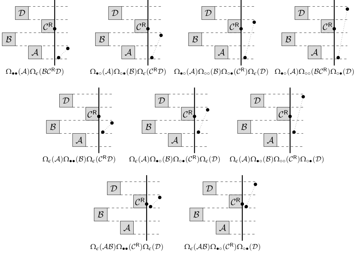
Figure 5: The expansion of \Omega_{\bullet\bullet}(\mathcal{C}) given the equation \mathcal{C} = ABC^R D is given by the combinatorial sum of the 9 terms above.
