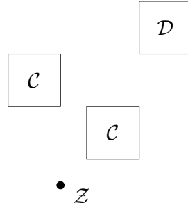
Figure 2: An example of a class which would correspond to the term ZCCD in a bottom-to-top combinatorial specification.
