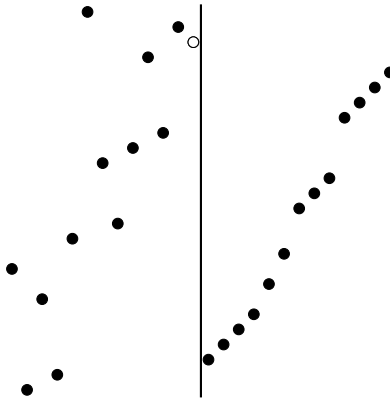
Figure 3: The role of the rightmost point of the class \mathcal{C} in fixing a greedy gridding for \mathcal{C}|\mathcal{M} . A gridline any further left would produce a basis element of \mathcal{M} involving this entry.
