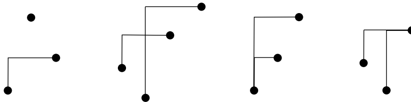
FIGURE 2. Four arrangements of hooks that are forbidden in a valid hook configuration.
