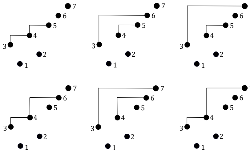
FIGURE 3. The valid hook configurations of 3142567.
