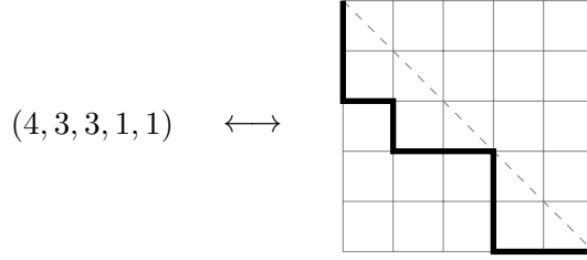
FIGURE 7. Dyck path corresponding to \alpha = (4, 3, 3, 1, 1) .
