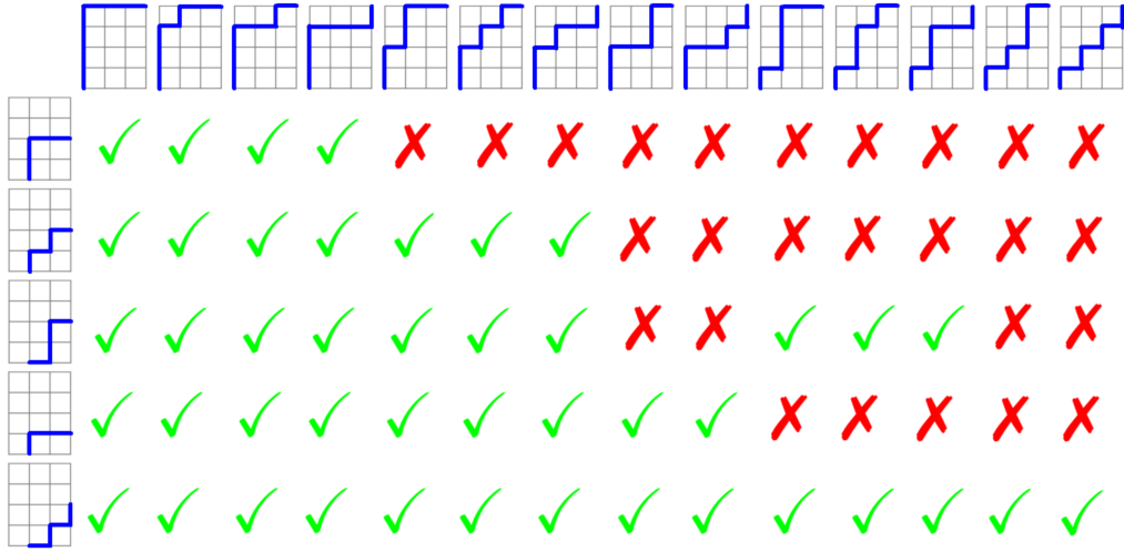
Figure 3. All non-intersecting lattice paths (green) associated to the point configuration A = \{(-3, 0), (-2, 0), (0, 0)\}, B = \{(0, 4), (0, 2), (0, 0)\}
