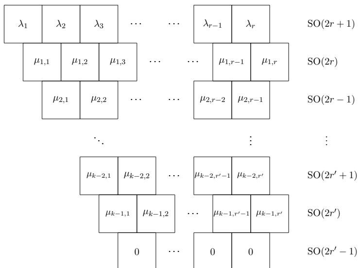
Figure 2. Gelfand-Tsetlin pattern of shape (SO(m), SO(n)) with n, m both odd
