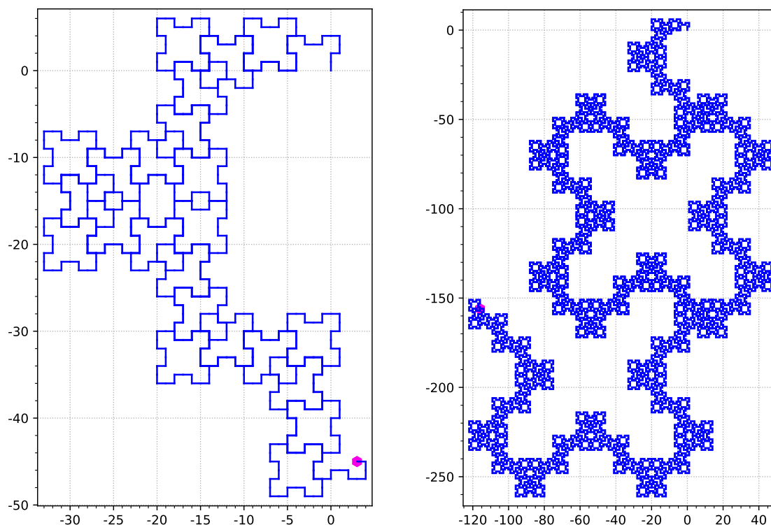
FIGURE 3. Fractal type curves generated by the odd-even drawing rule applied to the Sturmian word defined by the rotation R_{\sqrt{7}/7}(0.2) . The image on the left represents the trajectory after 1000 steps and the one on the right after 20000 steps (so the image on the left side can be found embedded in image on the right side).
