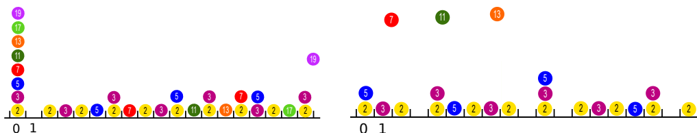
FIGURE 1. Two ways to fill the boxes of \mathcal{L} by pearls of primes. On the left, all primes are placed with a pearl in the zero box, exactly as in the sequence of integers, where the box one always remains unoccupied, while on the covering on the right side, primes 2 and 5 are also placed in the zero box, 3 is shifted to the right and three more boxes are ready to fit effectively the remaining primes 7, 11, 13 to generate the perfect minimal complete covering of the segment of length 17.
