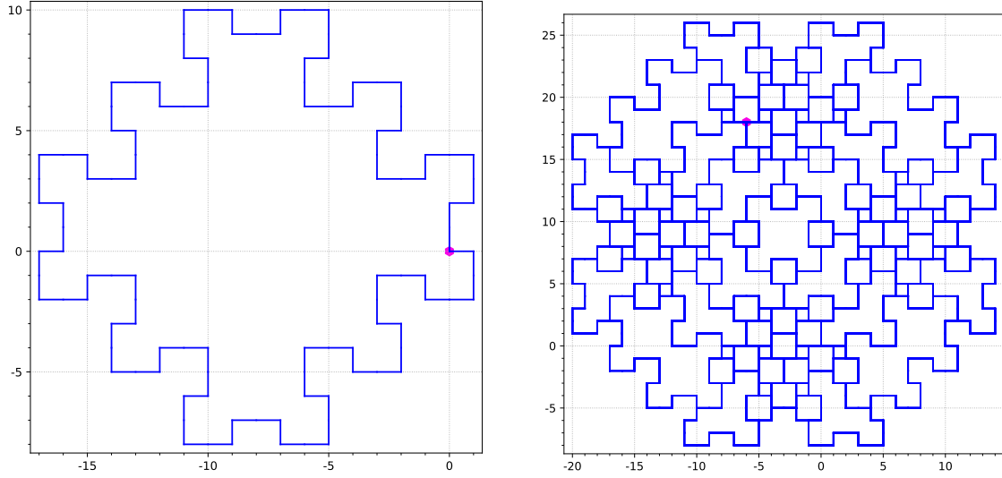
FIGURE 4. Fractal curves generated by the odd-even drawing rule applied to the Sturmian word defined by the rotation R_{\pi/8}(0.2) . The image on the left side represents the trajectory after 200 steps and the one on the right side is the continuation for a total of 20000 steps.
