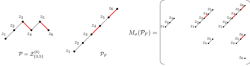
FIGURE 4. Left: a ribbon poset \mathcal{P} . Center: the folded ribbon \mathcal{P}_F . Right: its component array M_\sigma(\mathcal{P}_F) .
