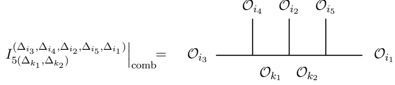
Fig. 2: Scalar five-point conformal blocks.
