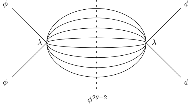
Figure 6.1: Feynman diagram for operators in the crossed channel, showing that the operator \phi^{2\theta-2} contributes at order \lambda^2 , or equivalently at order \epsilon^2 .
