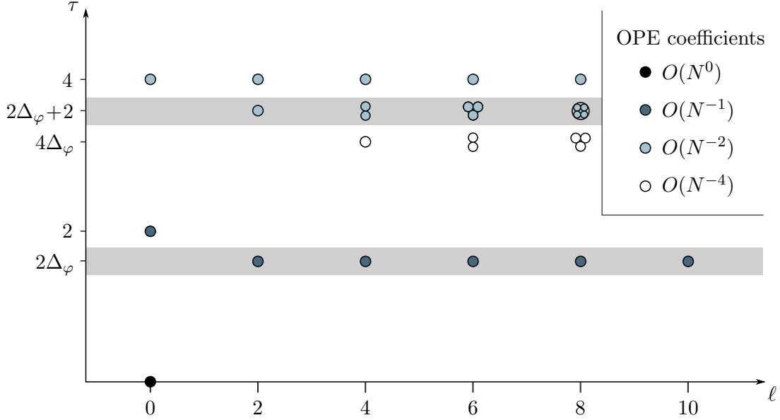
Figure 2.5: Operators, labels and mixing in the critical O(N) model at large N , displaying operators in the singlet representation.
