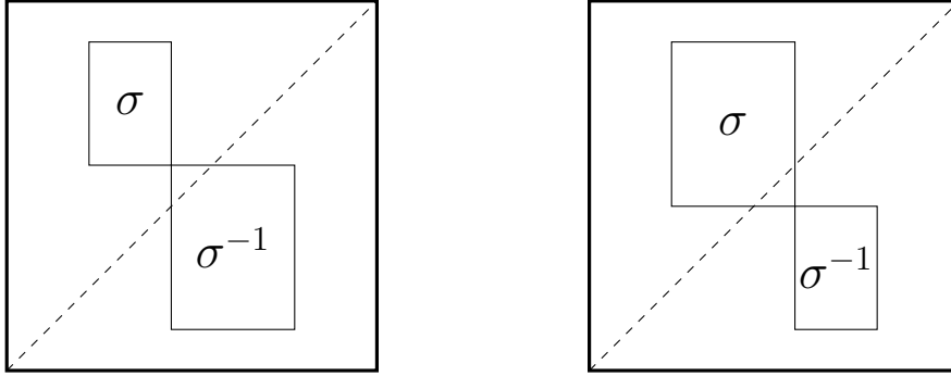
FIGURE 1. In the diagram on the left, all of \sigma lies above the main diagonal of \kappa . In the diagram on the right, all of \sigma^{-1} lies below the main diagonal. In these diagrams, we use different-sized rectangles to represent \sigma and \sigma^{-1} , not squares and not of equal size, to emphasize the fact that \sigma and \sigma^{-1} may be spread out across various entries of \kappa , both vertically and horizontally.
