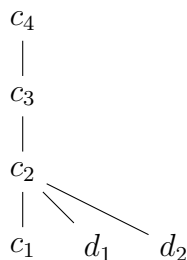
FIGURE 6. The poset H_{6,4} . The chain C = \{c_1, c_2, c_3, c_4\} of length 4 has 2 additional descendants added to the second-smallest element c_2 .
