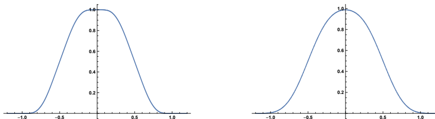
FIGURE 4. Plots of density functions for the distributions \mathcal{S}_{\mathbf{t}} with \mathbf{t} = (1, 1/2, 1/4, 1/8, 1/16, 1/32, 1/64, 1/128, 1/256) and \mathbf{t} = (1, 1/2, 1/3, 1/4, 1/5, 1/6, 1/7, 1/8, 1/9) .
