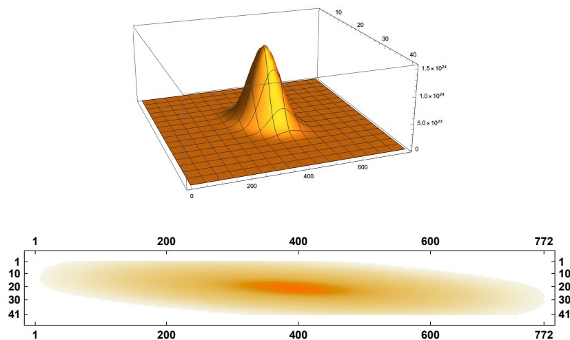
FIGURE 8. Plots of coefficients of the q, t -hook length formula (60) with \lambda = (25, 4, 3, 3, 1, 1, 1, 1, 1) .
