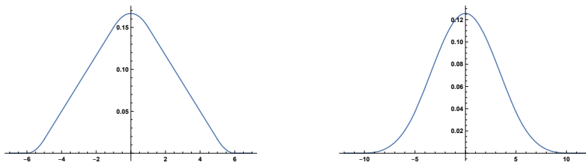
FIGURE 3. Plots of density functions for the distributions \mathcal{S}_{\mathbf{t}} with \mathbf{t} = (6, 5, 1) and \mathbf{t} = (6, 5, 5, 5, 1) .
