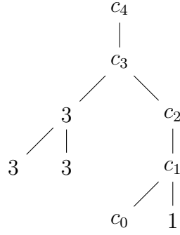
FIGURE 7. A tree P with maximal chain C = \{c_0 < c_1 < c_2 < c_3 < c_4\} and elevations of P - C labeled.
