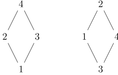
FIGURE 1. A naturally labeled poset (P, v) on the left and another labeling of the same diamond poset (P, w) on the right which is not natural or regular.
