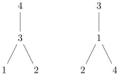
FIGURE 2. A naturally labeled poset (P, v) on the left and another labeling of the same forest poset (P, w) on the right which is not natural.
