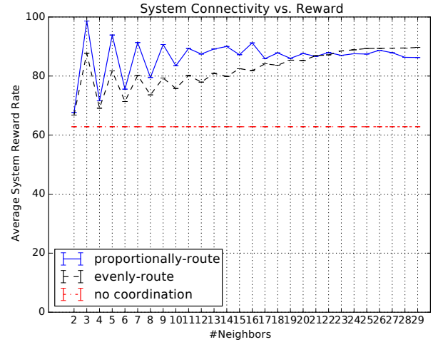
Figure 1: Utility Rate for a k -connected topology where the first half agents are heavily loaded and the other half are lightly loaded.
