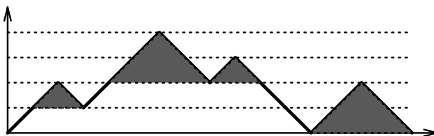
Figure 2.2: Maximal pyramids and exterior pairs in a Dyck path
