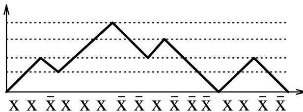
Figure 2.1: Example of a Dyck path and its associated Dyck word
