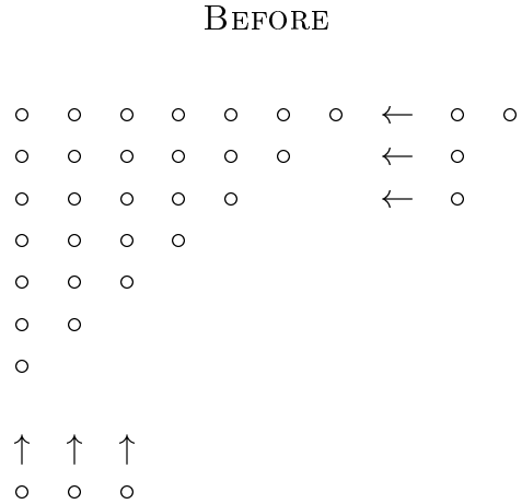
Figure 1. The Ferrars graph construction of Theorem 16 for m = 7 , a = 4 = 2+1+1 , and b = 3 = 1+1+1 , yielding the partition of T_7+7 = 35 = 9+7+6+4+3+3+2+1 with 7 distinct parts.
