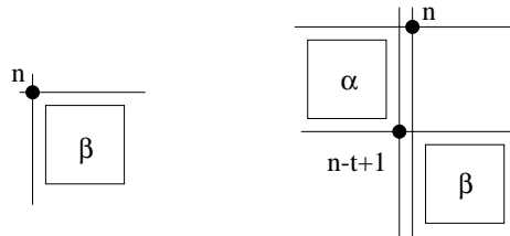
FIGURE 2. The block decomposition for \pi \in \mathfrak{M}_n .
