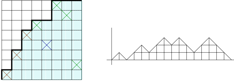
FIGURE 1. The bijection \varphi .
