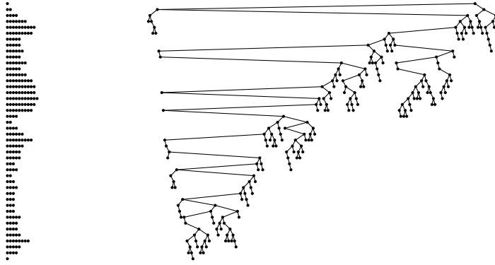
FIGURE 9. A random pruned binary tree of size 256 and its associated level profile: the histogram on the left displays the number of nodes at each level in the tree.
