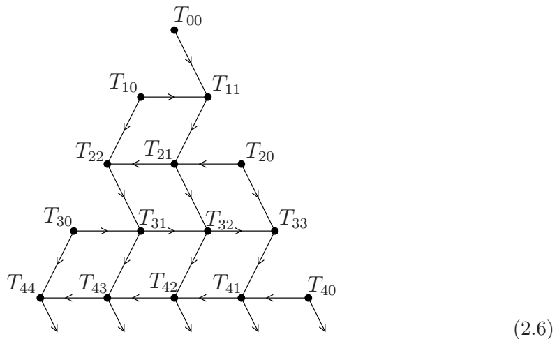
Figure 1: Directed graph \Gamma underlying the boustrophedon transform.
