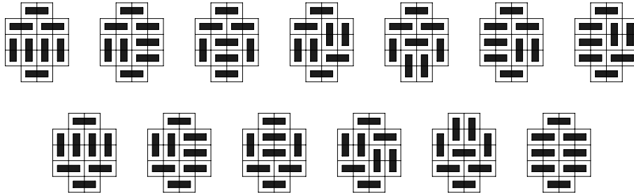
FIGURE 12. d_2 tilings.
