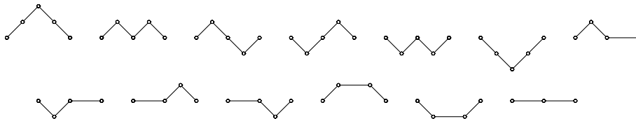
FIGURE 1. The d_2 = 13 unrestricted paths from (0, 0) to (2n, 0) using the steps U , D , and (2, 0) .
