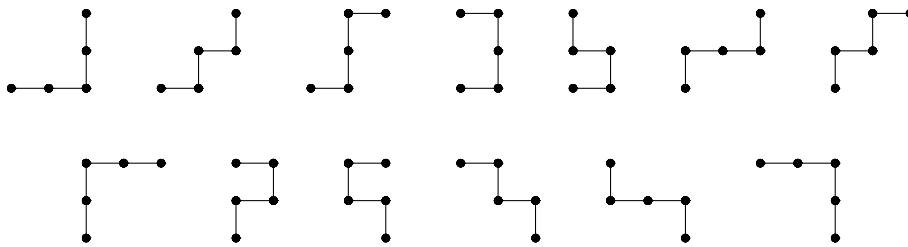
FIGURE 15. d_2 walks.
