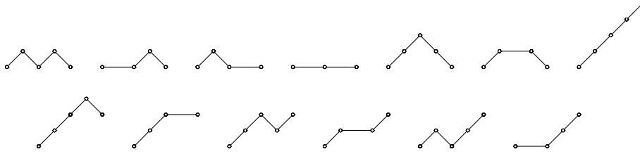
FIGURE 19. The paths running from (0,0) to the line x = 4 and remaining weakly above the x-axis.
