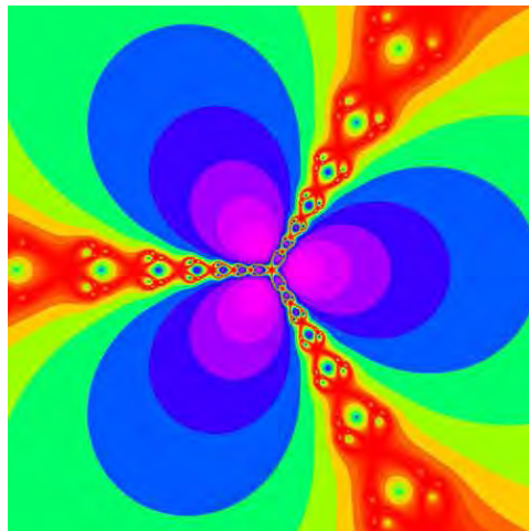
A Julia set
