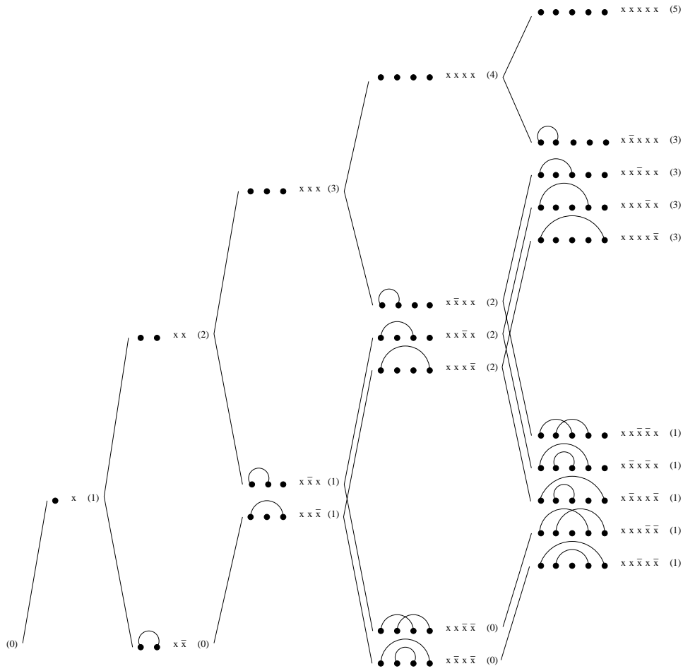
FIGURE 1. The generating trees of the 132-avoiding involutions and the Dyck word prefixes, with the labels of the succession system which characterizes them.
