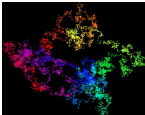
Figure 2: A walk on the base-4 digits of \pi .
